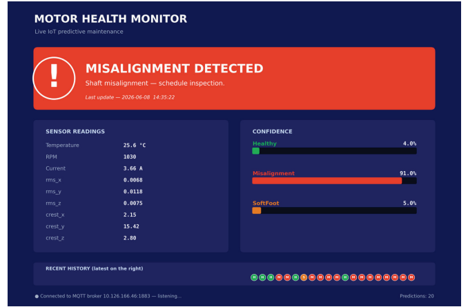
Fig. 7. Real-time monitoring dashboard showing the detected motor condition, confidence values, live sensor readings, and prediction history.
