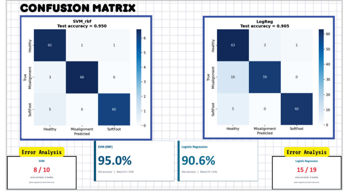
Fig. 6. Confusion matrices and test accuracies for SVM with RBF kernel and logistic regression classifiers.
