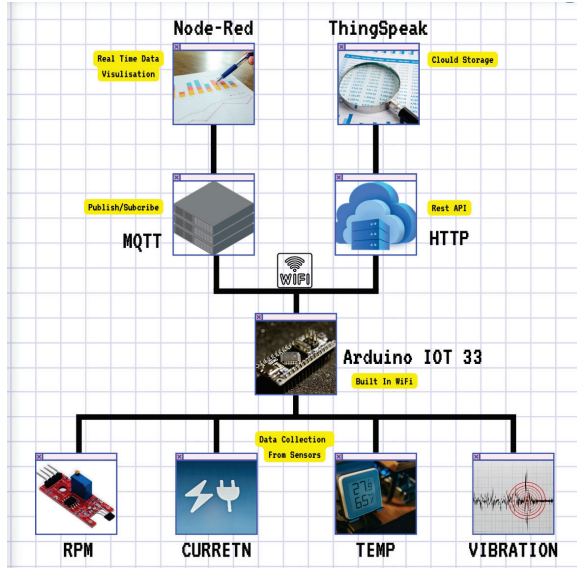
Fig. 2. Communication architecture using MQTT for local real-time monitoring and HTTP/ThingSpeak for cloud data logging.
