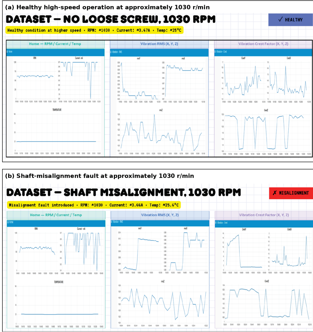
Fig. 3. Representative experimental dashboard outputs for two high-speed test cases: (a) healthy operation and (b) shaft-misalignment fault, both at approximately 1030 r/min. The comparison shows that current and surface temperature remained similar, while the vibration RMS and crest-factor responses changed more clearly under misalignment.
