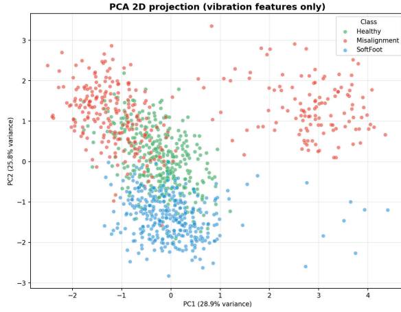
Fig. 5. PCA projection of the six standardised vibration features. The first two principal components explain 54.7% of the variance.
