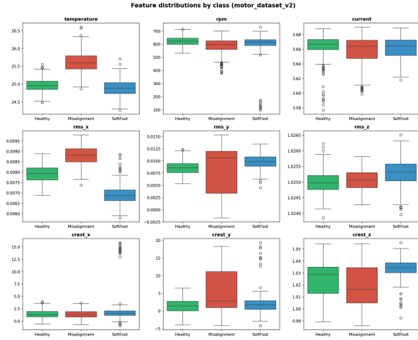
Fig. 4. Boxplots of the measured features showing class-dependent variation in vibration features.
